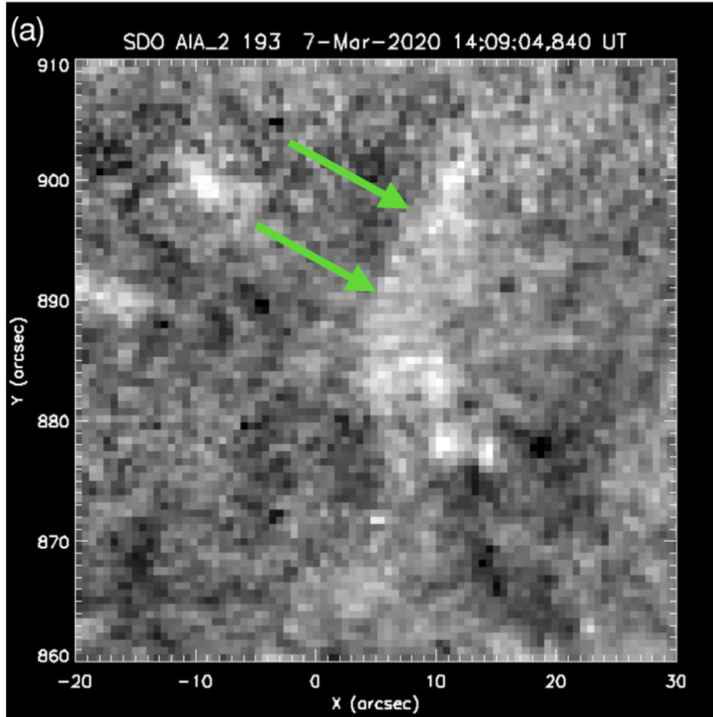
Figure 4. from Alphonse C. Sterling et al 2022 Astrophys. J. 940 doi:10.3847/1538-4357/ac9960 http://dx.doi.org/10.3847/1538-4357/ac9960 © 2022. The Author(s). Published by the American Astronomical Society.
