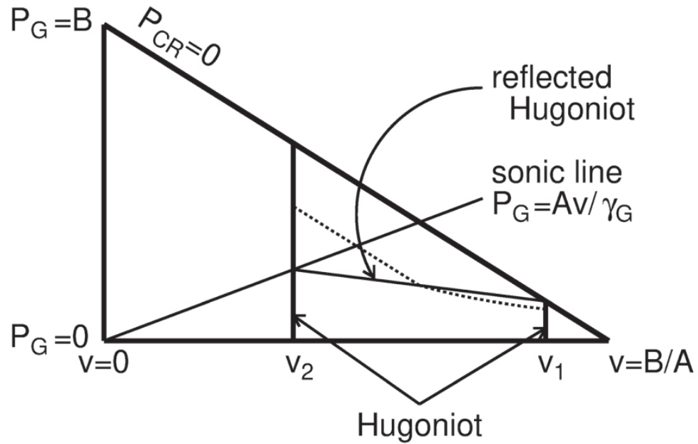
Figure 4. from J. Martin Laming 2022 Astrophys. J. 940 doi:10.3847/1538-4357/ac98bb https://dx.doi.org/10.3847/1538-4357/ac98bb © 2022. The Author(s). Published by the American Astronomical Society.
