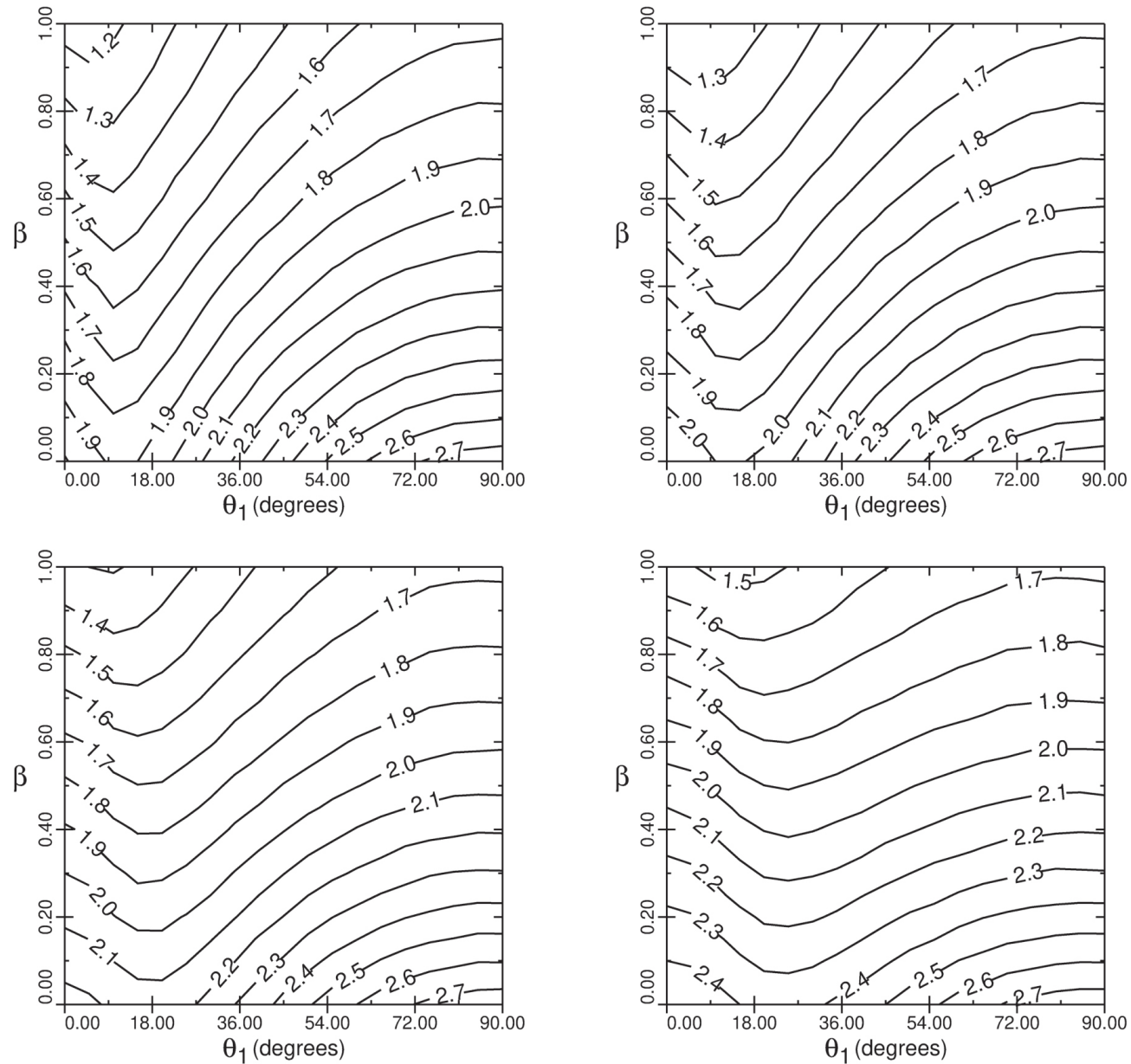
Figure 2. from J. Martin Laming 2022 Astrophys. J. 940 doi:10.3847/1538-4357/ac98bb https://dx.doi.org/10.3847/1538-4357/ac98bb © 2022. The Author(s). Published by the American Astronomical Society.
