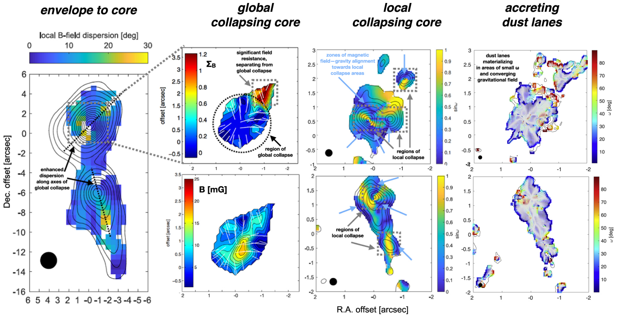
Figure 9. from Patrick M. Koch et al 2022 Astrophys. J. 940 doi:10.3847/1538-4357/ac96e3 http://dx.doi.org/10.3847/1538-4357/ac96e3 © 2022. The Author(s). Published by the American Astronomical Society.
