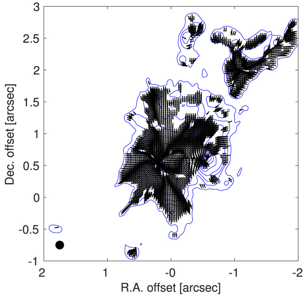
Figure 4. from Patrick M. Koch et al 2022 Astrophys. J. 940 doi:10.3847/1538-4357/ac96e3 http://dx.doi.org/10.3847/1538-4357/ac96e3 © 2022. The Author(s). Published by the American Astronomical Society.
