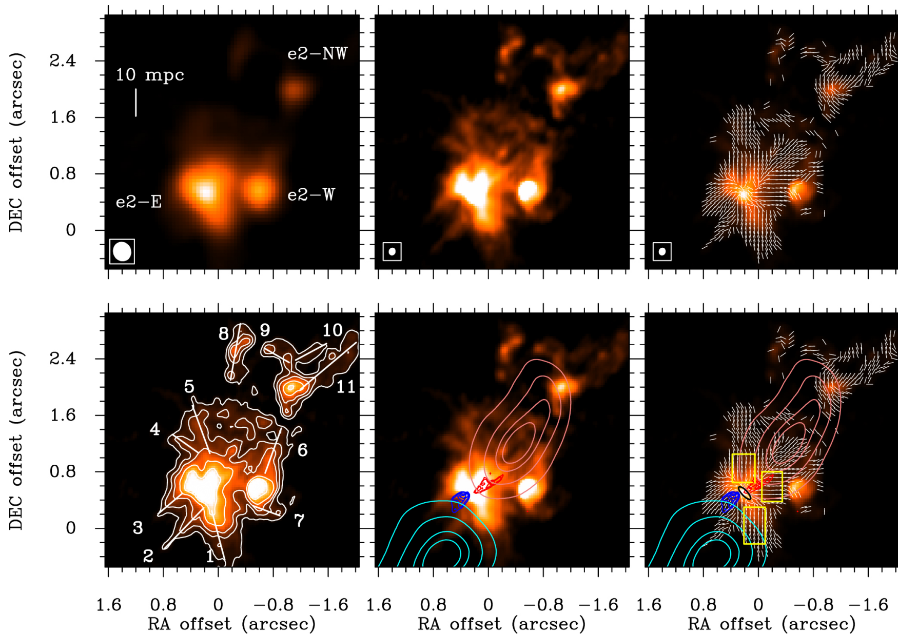
Figure 1. from Patrick M. Koch et al 2022 Astrophys. J. 940 doi:10.3847/1538-4357/ac96e3 https://dx.doi.org/10.3847/1538-4357/ac96e3 © 2022. The Author(s). Published by the American Astronomical Society.
