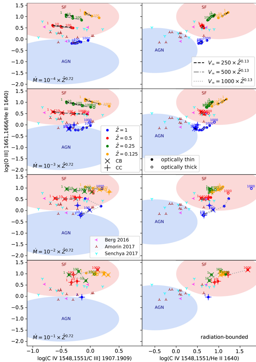
Figure 9. from Ashkbiz Danehkar et al 2021 Astrophys. J. 921 doi:10.3847/1538-4357/ac1a76 https://dx.doi.org/10.3847/1538-4357/ac1a76 © 2021. The American Astronomical Society. All rights reserved.
