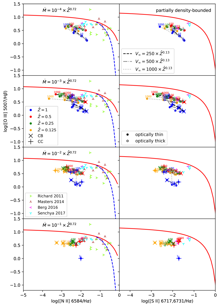
Figure 8. from Ashkbiz Danehkar et al 2021 Astrophys. J. 921 doi:10.3847/1538-4357/ac1a76 https://dx.doi.org/10.3847/1538-4357/ac1a76 © 2021. The American Astronomical Society. All rights reserved.
