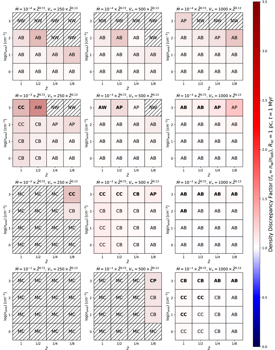
Figure 5. from Ashkbiz Daneshkar et al 2021 Astrophys. J. 921 doi:10.3847/1538-4357/ac1a76 https://dx.doi.org/10.3847/1538-4357/ac1a76 © 2021. The American Astronomical Society. All rights reserved.
