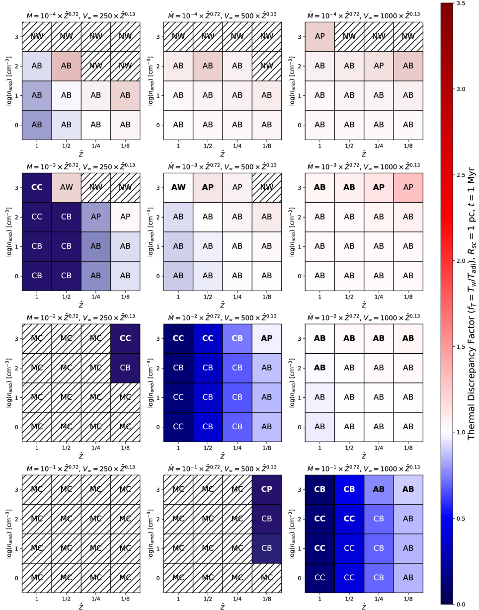
Figure 4. from Ashkbiz Daneshkar et al 2021 Astrophys. J. 921 doi:10.3847/1538-4357/ac1a76 https://dx.doi.org/10.3847/1538-4357/ac1a76 © 2021. The American Astronomical Society. All rights reserved.
