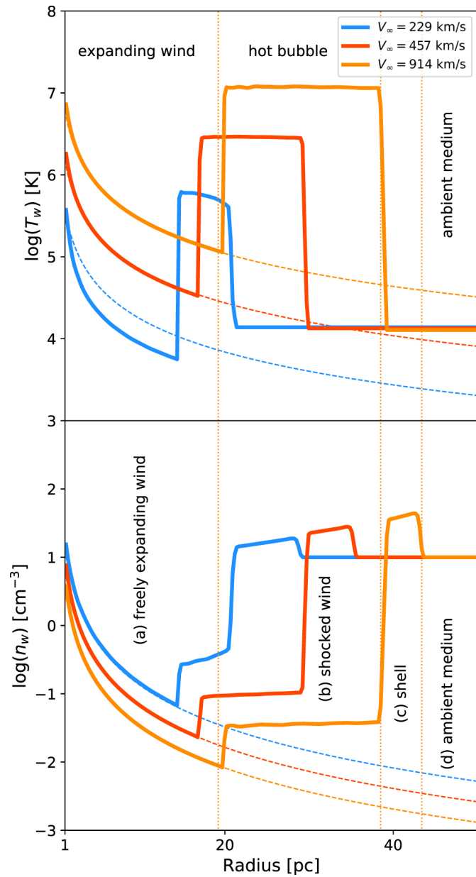
Figure 2. from Ashkbiz Danehkar et al 2021 Astrophys. J. 921 doi:10.3847/1538-4357/ac1a76 https://dx.doi.org/10.3847/1538-4357/ac1a76 © 2021. The American Astronomical Society. All rights reserved.
