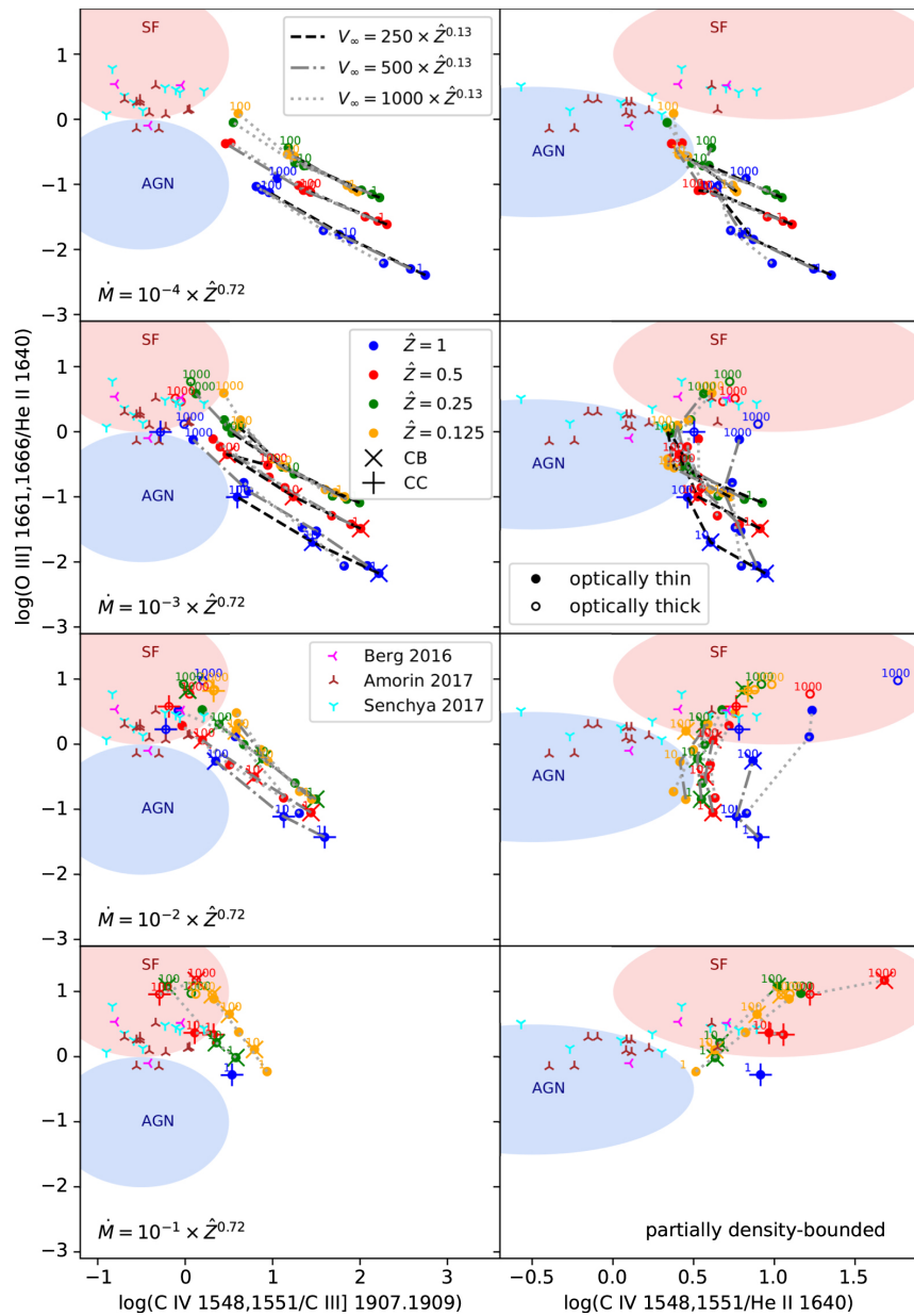
Figure 10. from Ashkbiz Danehkar et al 2021 Astrophys. J. 921 doi:10.3847/1538-4357/ac1a76 https://dx.doi.org/10.3847/1538-4357/ac1a76 © 2021. The American Astronomical Society. All rights reserved.
