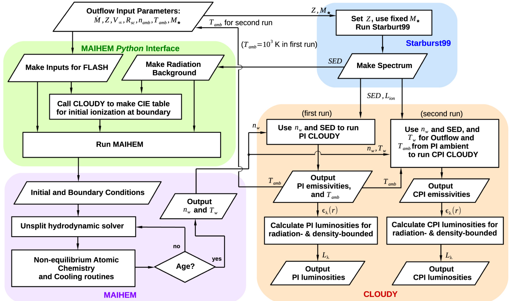
Figure 1. from Ashkbiz Daneshkar et al 2021 Astrophys. J. 921 doi:10.3847/1538-4357/ac1a76 https://dx.doi.org/10.3847/1538-4357/ac1a76 © 2021. The American Astronomical Society. All rights reserved.
