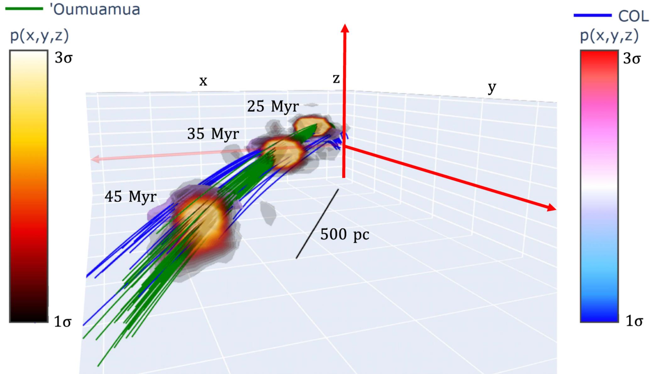
Figure 4. from Evidence Suggesting That 'Oumuamua Is the 30 Myr Old Product of a Molecular Cloud null 2021 APJ 917 20 doi:10.3847/1538-4357/ac0729 https://dx.doi.org/10.3847/1538-4357/ac0729 © 2021. The American Astronomical Society. All rights reserved.
