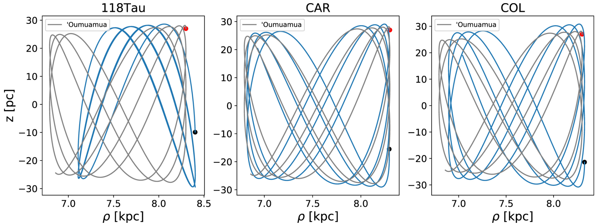
Figure 3. from Evidence Suggesting That 'Oumuamua Is the 30 Myr Old Product of a Molecular Cloud null 2021 APJ 917 20 doi:10.3847/1538-4357/ac0729 https://dx.doi.org/10.3847/1538-4357/ac0729 © 2021. The American Astronomical Society. All rights reserved.
