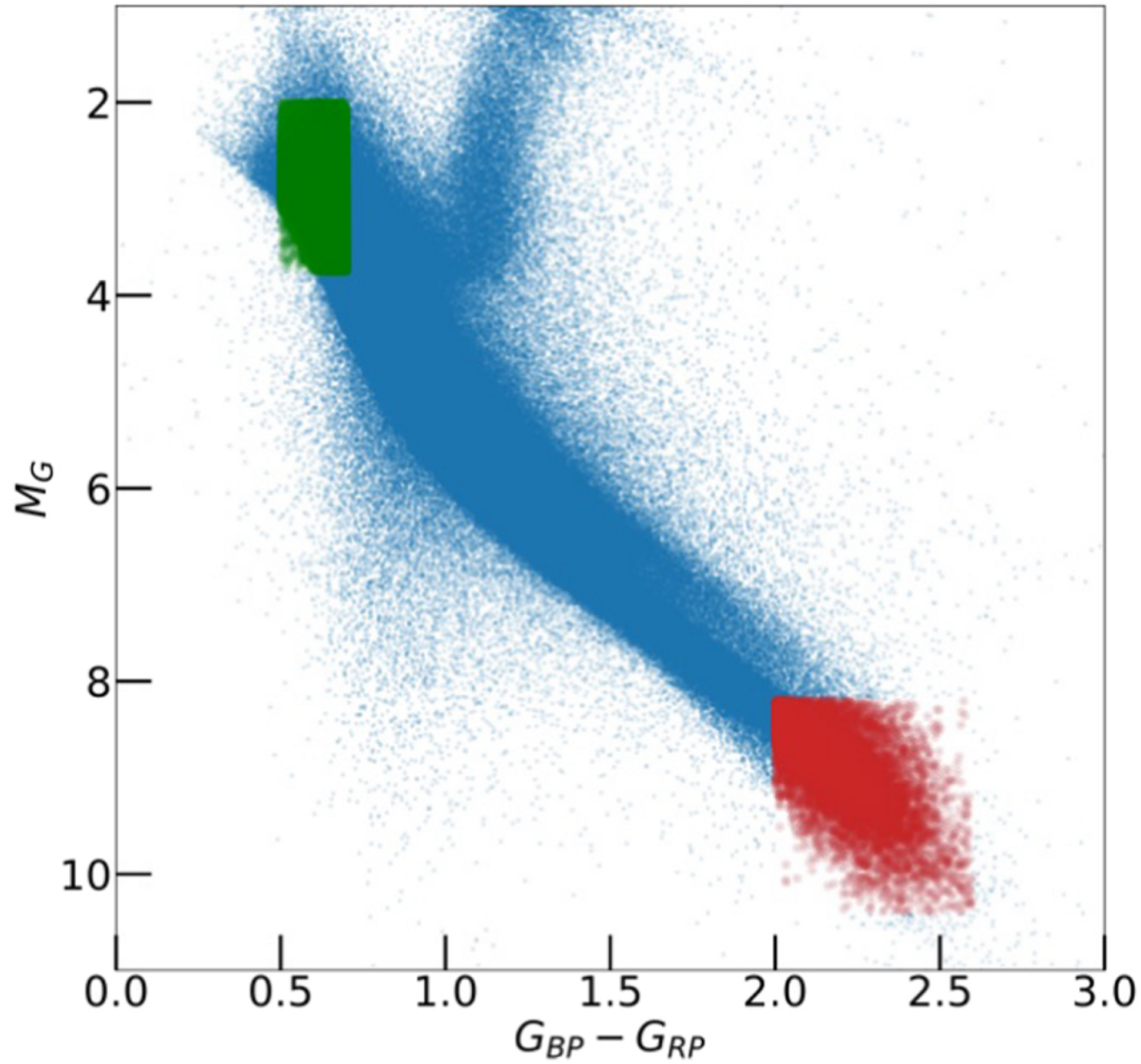
Figure 2. from Evidence Suggesting That 'Oumuamua Is the 30 Myr Old Product of a Molecular Cloud null 2021 APJ 917 20 doi:10.3847/1538-4357/ac0729 https://dx.doi.org/10.3847/1538-4357/ac0729 © 2021. The American Astronomical Society. All rights reserved.
