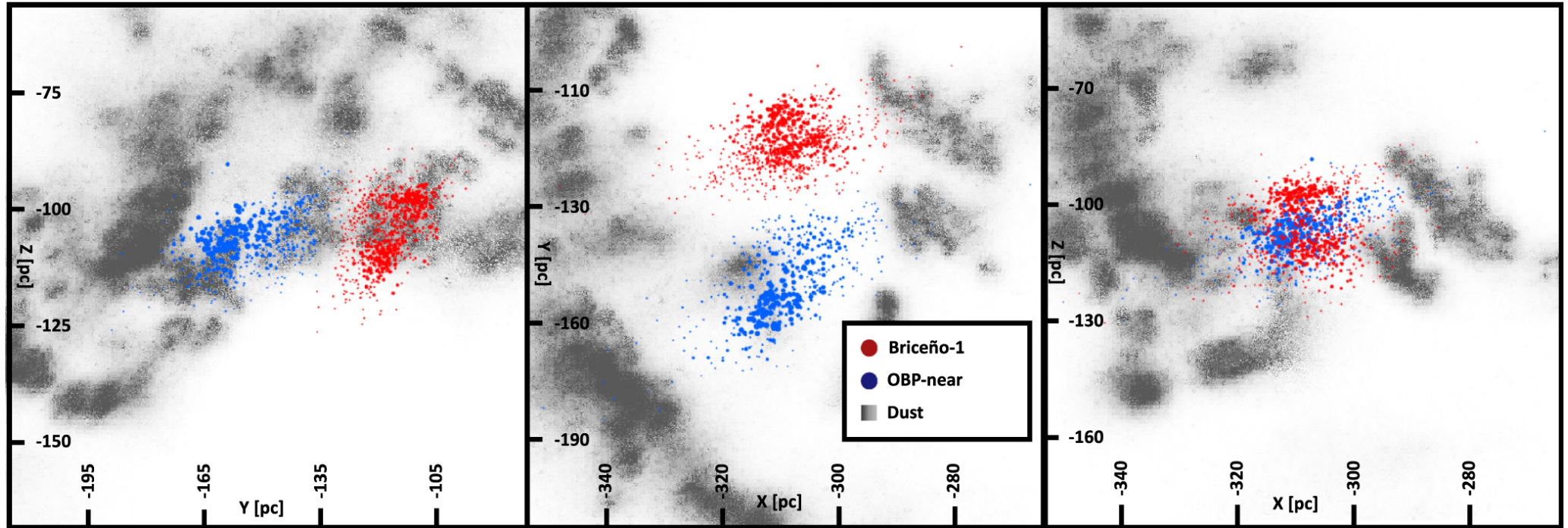
Figure 5. from Evidence for Radial Expansion at the Core of the Orion Complex with Gaia EDR3 null 2021 APJ 917 21 doi:10.3847/1538-4357/ac0633 https://dx.doi.org/10.3847/1538-4357/ac0633 © 2021. The American Astronomical Society. All rights reserved.
