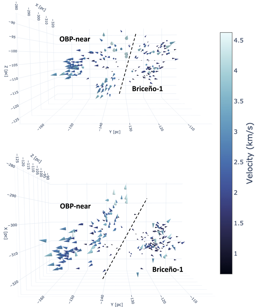
Figure 2. from Evidence for Radial Expansion at the Core of the Orion Complex with Gaia EDR3 null 2021 APJ 917 21 doi:10.3847/1538-4357/ac0633 https://dx.doi.org/10.3847/1538-4357/ac0633 © 2021. The American Astronomical Society. All rights reserved.
