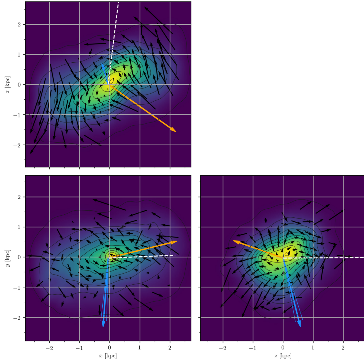
Figure 9. from Revealing the Structure and Internal Rotation of the Sagittarius Dwarf Spheroidal Galaxy with Gaia and Machine Learning null 2021 APJ 908 244 doi:10.3847/1538-4357/abd5bf https://dx.doi.org/10.3847/1538-4357/abd5bf © 2021. The American Astronomical Society. All rights reserved.
