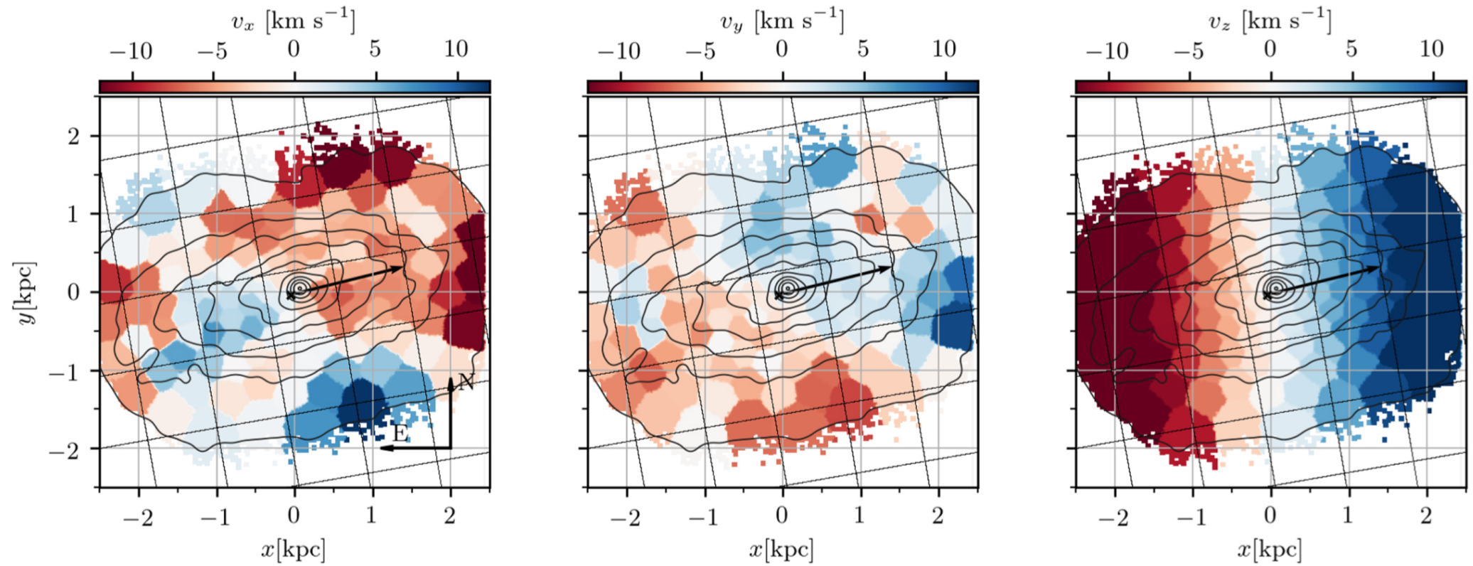
Figure 8. from Revealing the Structure and Internal Rotation of the Sagittarius Dwarf Spheroidal Galaxy with Gaia and Machine Learning null 2021 APJ 908 244 doi:10.3847/1538-4357/abd5bf https://dx.doi.org/10.3847/1538-4357/abd5bf © 2021. The American Astronomical Society. All rights reserved.
