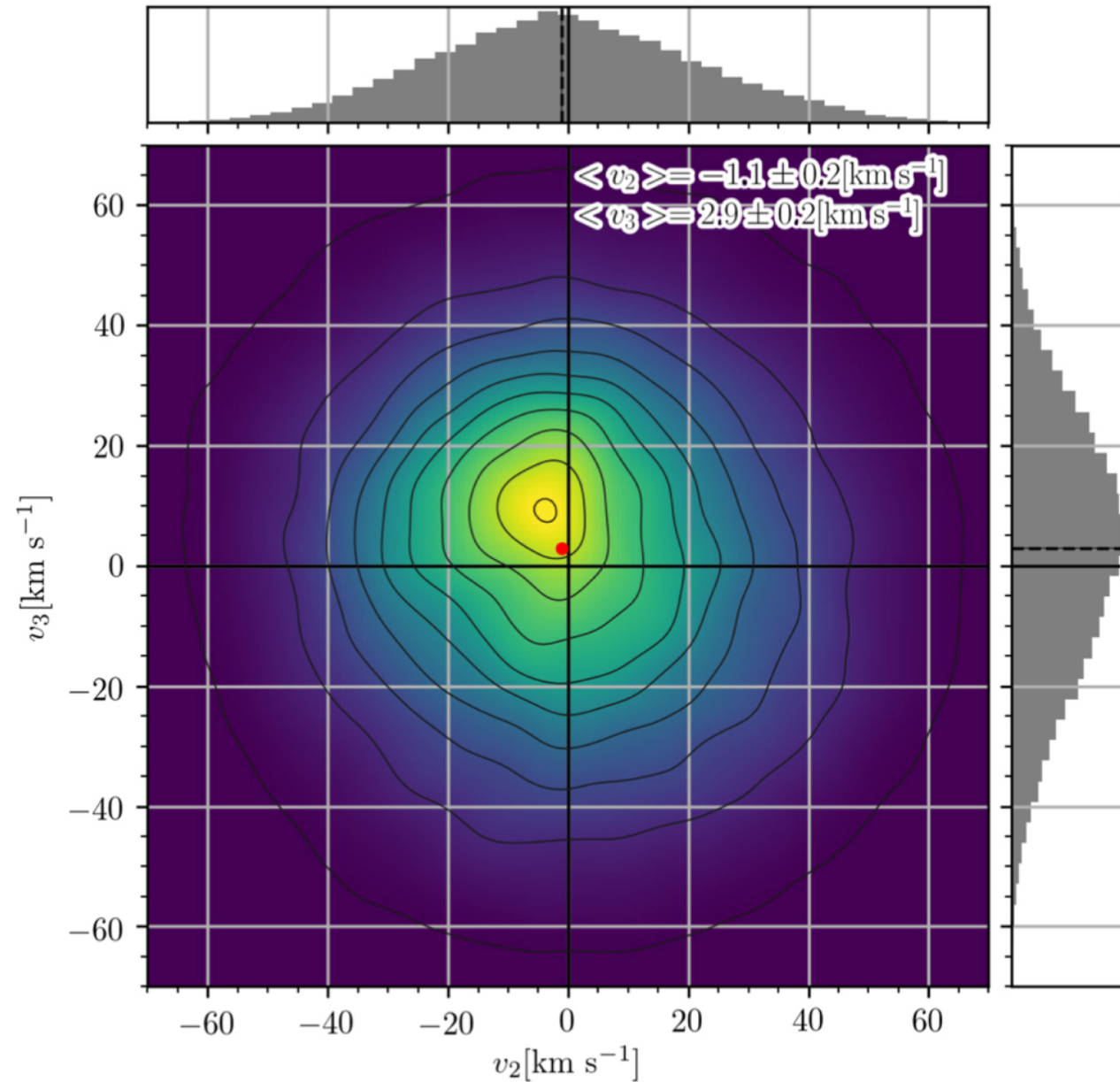
Figure 7. from Revealing the Structure and Internal Rotation of the Sagittarius Dwarf Spheroidal Galaxy with Gaia and Machine Learning null 2021 APJ 908 244 doi:10.3847/1538-4357/abd5bf https://dx.doi.org/10.3847/1538-4357/abd5bf © 2021. The American Astronomical Society. All rights reserved.
