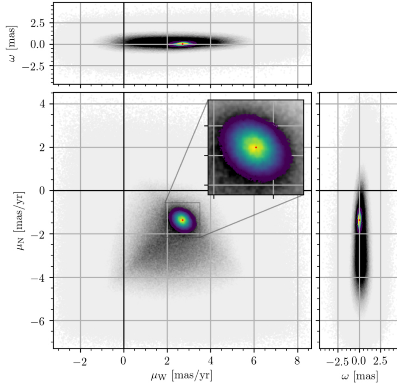
Figure 6. from Revealing the Structure and Internal Rotation of the Sagittarius Dwarf Spheroidal Galaxy with Gaia and Machine Learning null 2021 APJ 908 244 doi:10.3847/1538-4357/abd5bf https://dx.doi.org/10.3847/1538-4357/abd5bf © 2021. The American Astronomical Society. All rights reserved.
