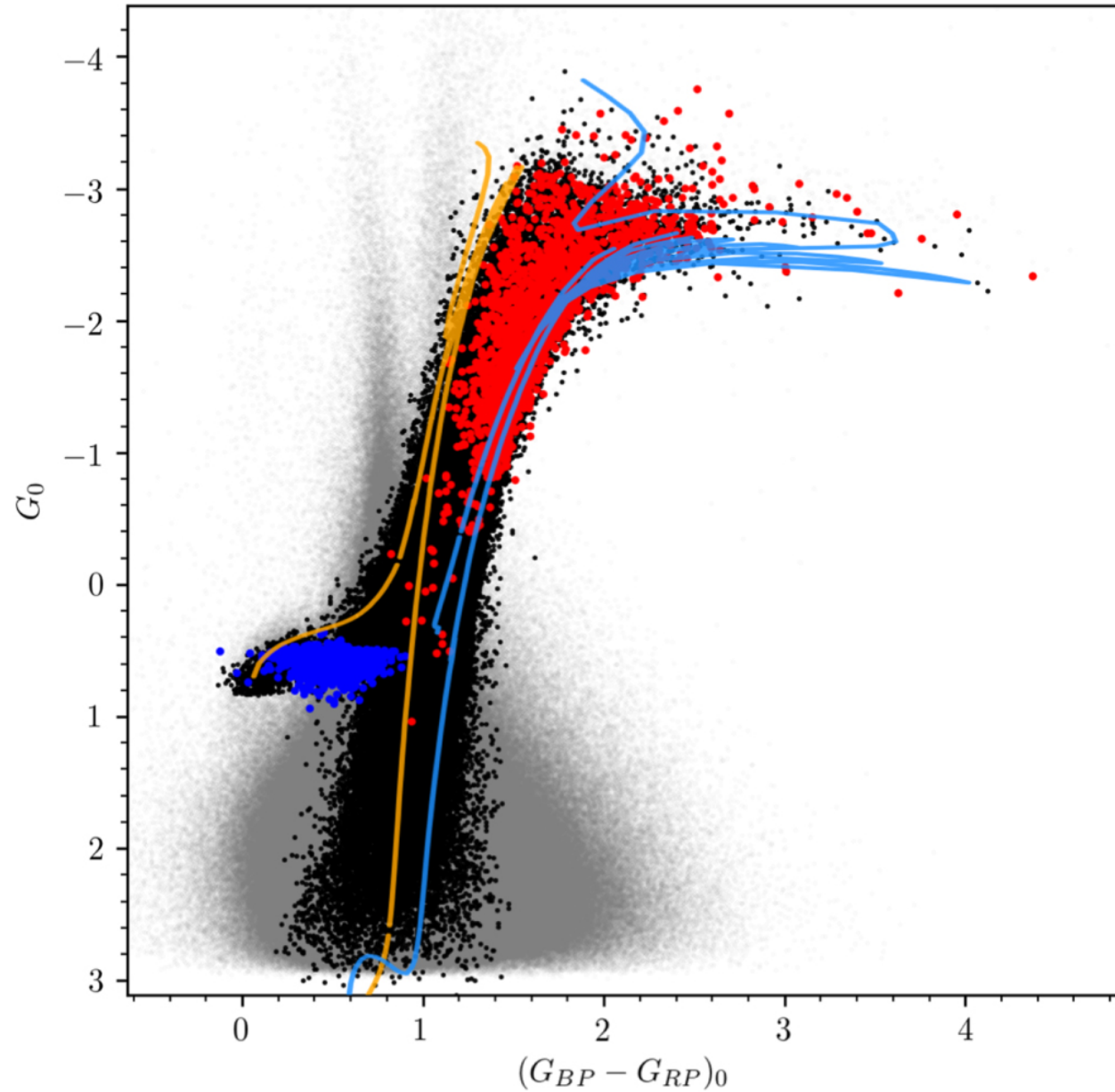
Figure 5. from Revealing the Structure and Internal Rotation of the Sagittarius Dwarf Spheroidal Galaxy with Gaia and Machine Learning null 2021 APJ 908 244 doi:10.3847/1538-4357/abd5bf https://dx.doi.org/10.3847/1538-4357/abd5bf © 2021. The American Astronomical Society. All rights reserved.
