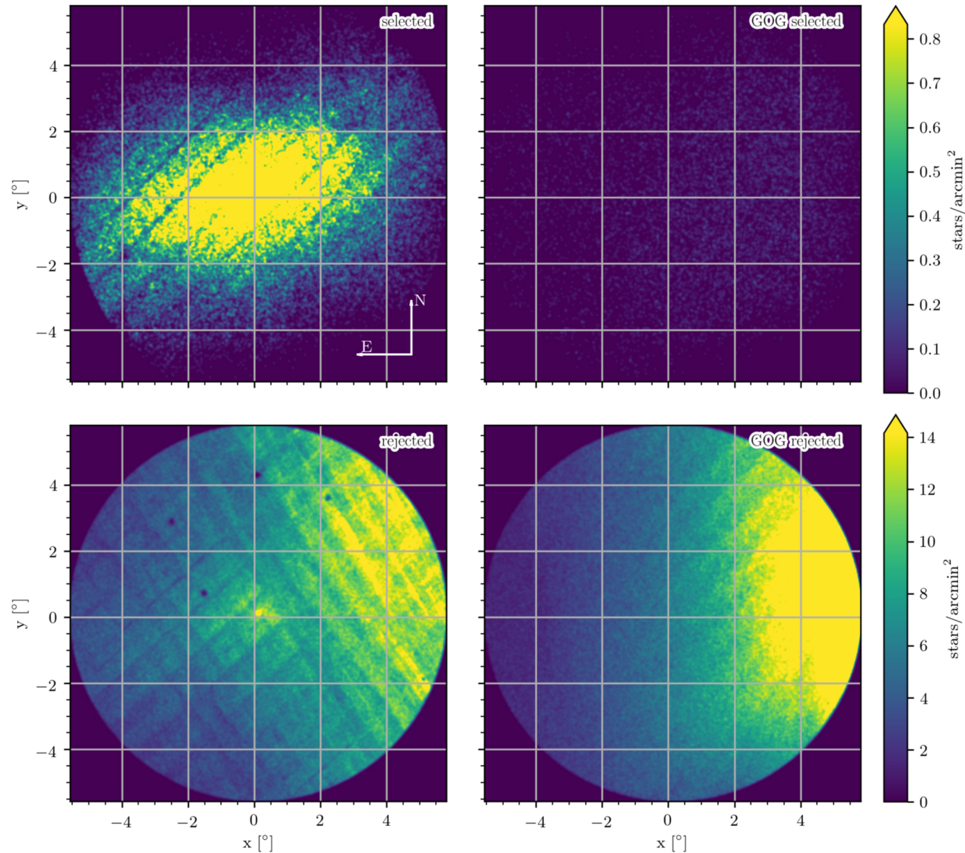
Figure 4. from Revealing the Structure and Internal Rotation of the Sagittarius Dwarf Spheroidal Galaxy with Gaia and Machine Learning null 2021 APJ 908 244 doi:10.3847/1538-4357/abd5bf https://dx.doi.org/10.3847/1538-4357/abd5bf © 2021. The American Astronomical Society. All rights reserved.
