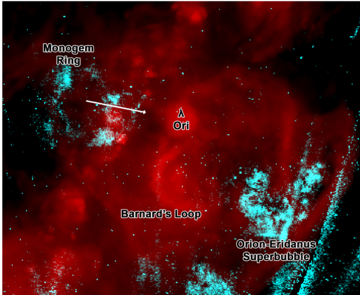
Figure 4. from Supernovae in Orion: The Missing Link in the Star-forming History of the Region null 2020 APJ 902 122 doi:10.3847/1538-4357/abb6e8 https://dx.doi.org/10.3847/1538-4357/abb6e8 © 2020. The American Astronomical Society. All rights reserved.
