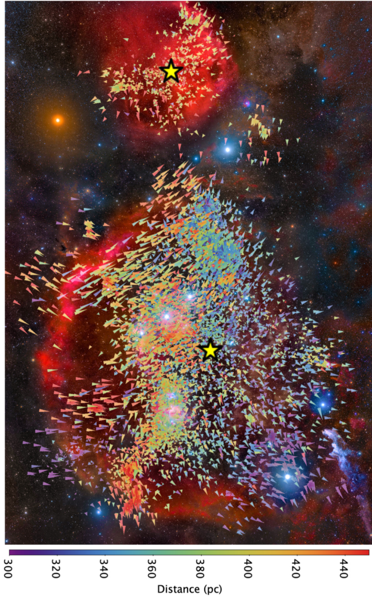
Figure 1. from Supernovae in Orion: The Missing Link in the Star-forming History of the Region null 2020 APJ 902 122 doi:10.3847/1538-4357/abb6e8 https://dx.doi.org/10.3847/1538-4357/abb6e8 © 2020. The American Astronomical Society. All rights reserved.
