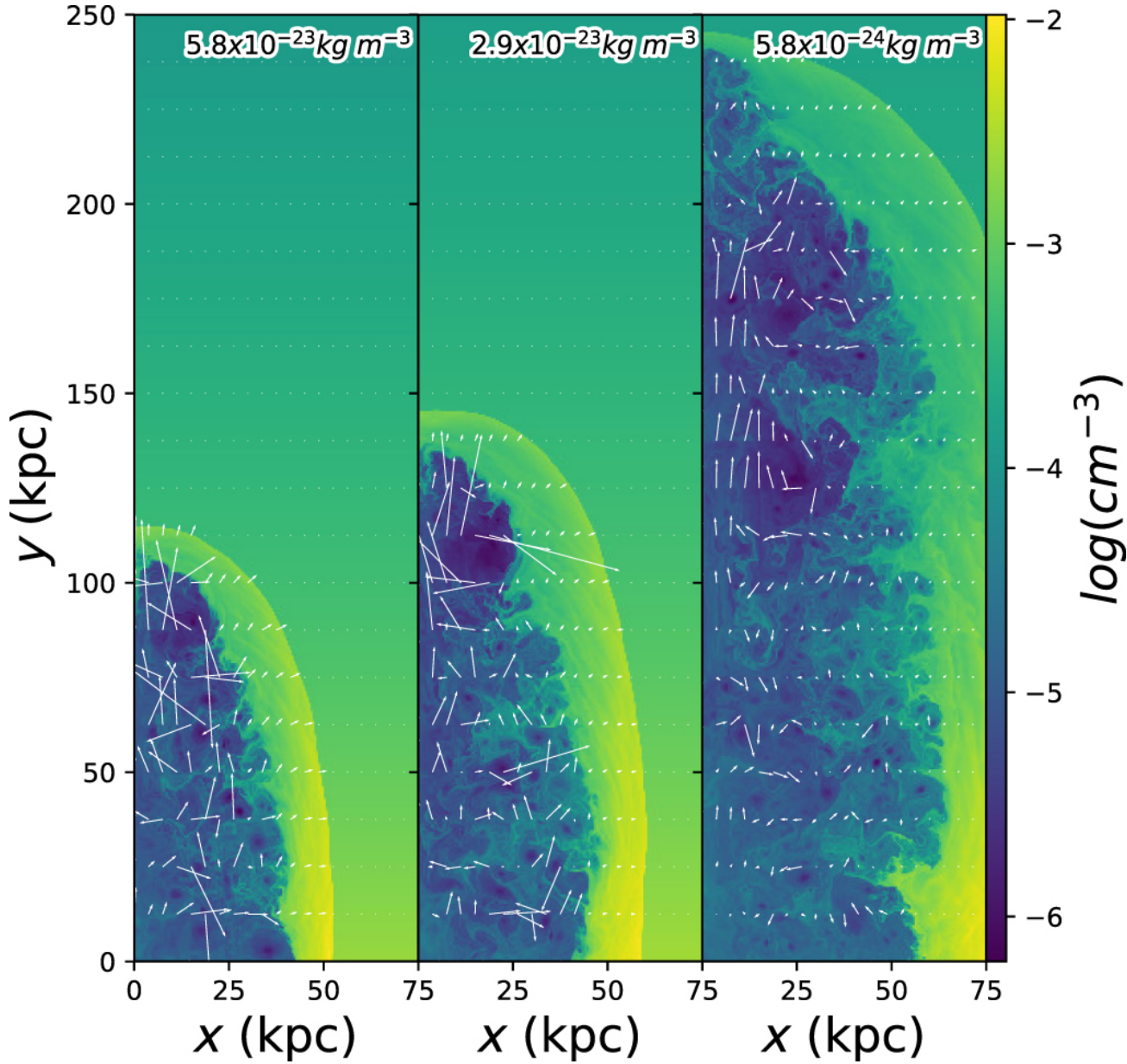
Figure 5. from Extended Radio AGN at z = 1 in the ORELSE Survey: The Confining Effect of Dense Environments null 2020 APJ 902 101 doi:10.3847/1538-4357/abb5a0 http://dx.doi.org/10.3847/1538-4357/abb5a0 © 2020. The American Astronomical Society. All rights reserved.
