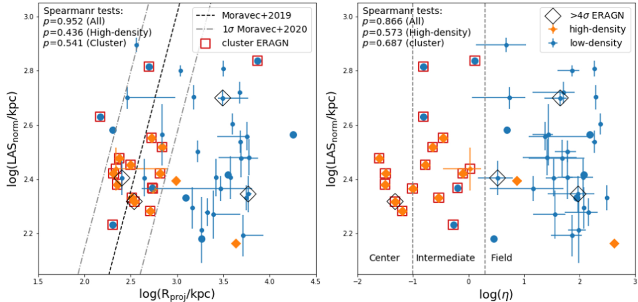
Figure 4. from Extended Radio AGN at z \sim 1 in the ORELSE Survey: The Confining Effect of Dense Environments null 2020 APJ 902 101 doi:10.3847/1538-4357/abb5a0 https://dx.doi.org/10.3847/1538-4357/abb5a0 © 2020. The American Astronomical Society. All rights reserved.
