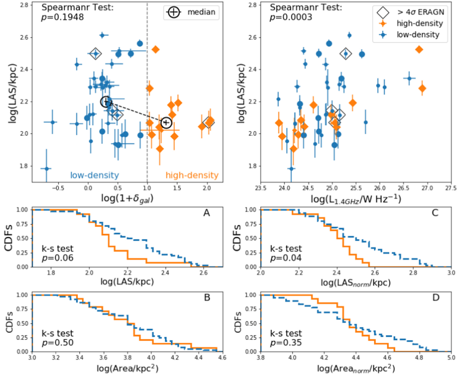
Figure 3. from Extended Radio AGN at z = 1 in the ORELSE Survey: The Confining Effect of Dense Environments null 2020 APJ 902 101 doi:10.3847/1538-4357/abb5a0 http://dx.doi.org/10.3847/1538-4357/abb5a0 © 2020. The American Astronomical Society. All rights reserved.
