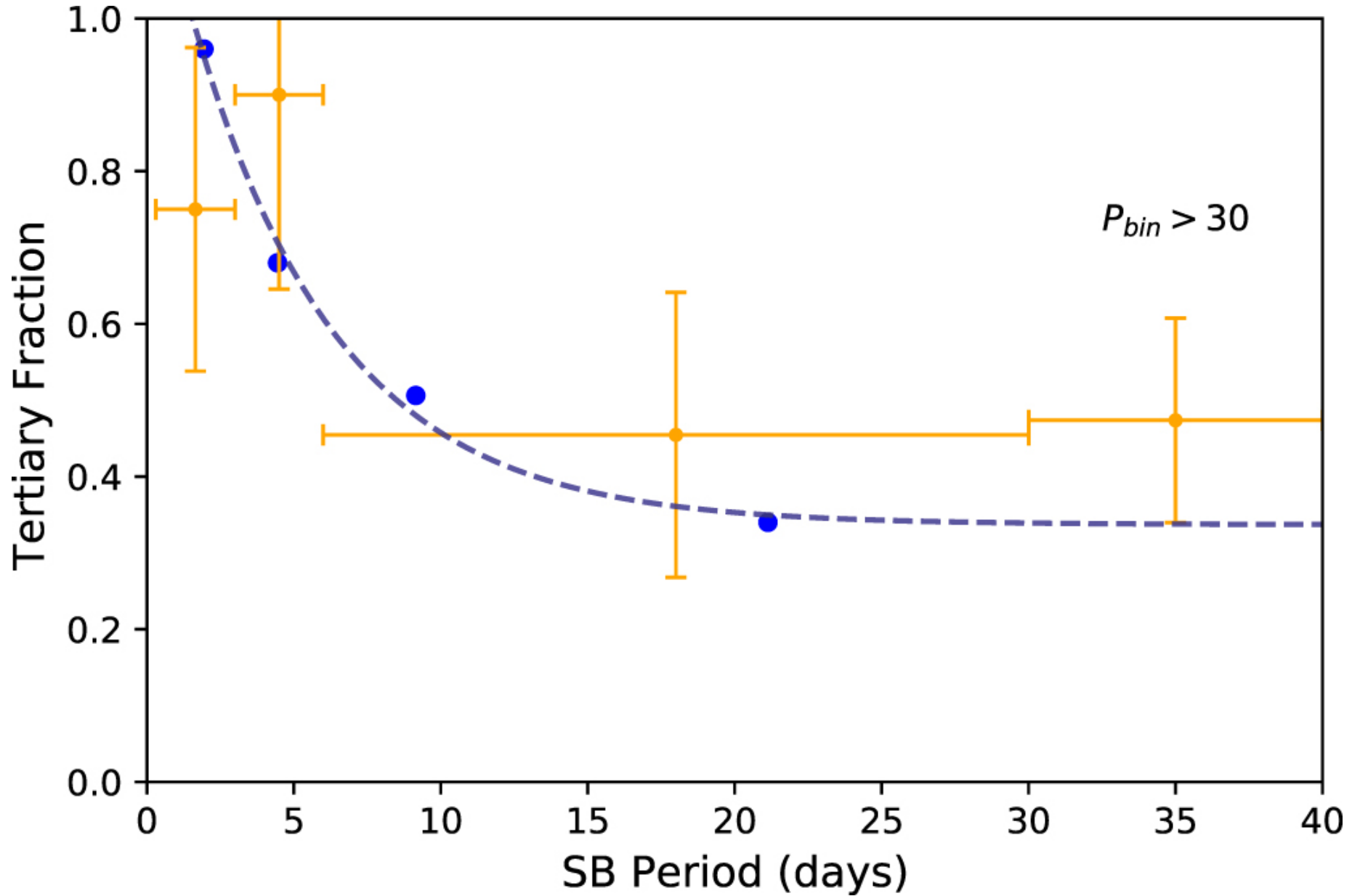
Figure 5. from Assessing Spectroscopic Binary Multiplicity Properties Using Robo-AO Imaging null 2020 APJ 902 107 doi:10.3847/1538-4357/abb3fe http://dx.doi.org/10.3847/1538-4357/abb3fe © 2020. The American Astronomical Society. All rights reserved.
