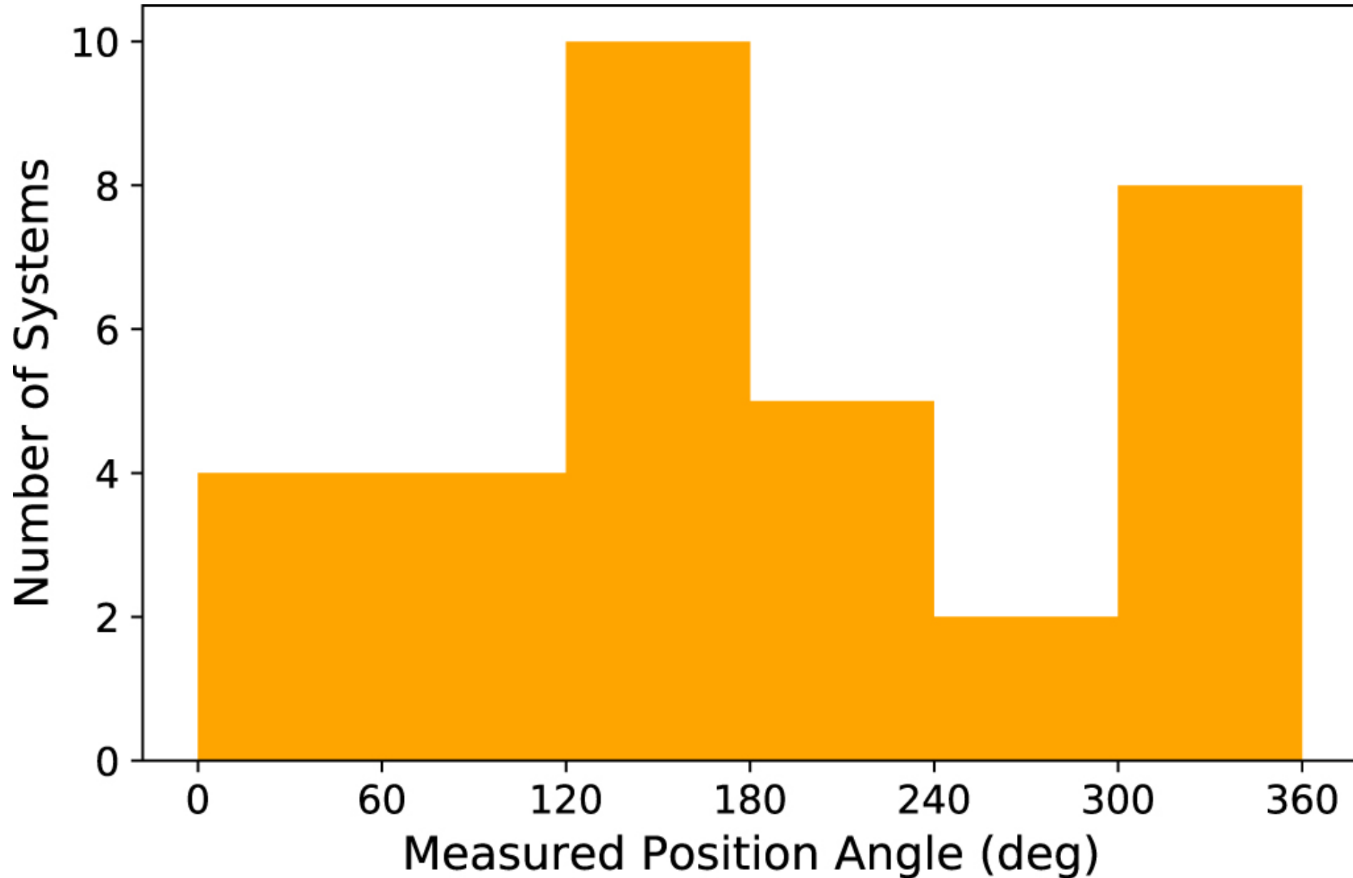
Figure 3. from Assessing Spectroscopic Binary Multiplicity Properties Using Robo-AO Imaging null 2020 APJ 902 107 doi:10.3847/1538-4357/abb3fe http://dx.doi.org/10.3847/1538-4357/abb3fe © 2020. The American Astronomical Society. All rights reserved.
