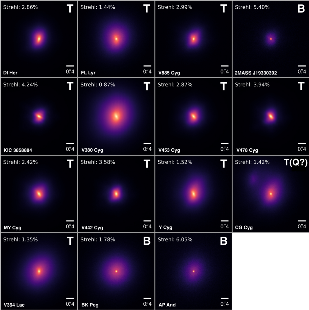
Figure 11. from Assessing Spectroscopic Binary Multiplicity Properties Using Robo-AO Imaging null 2020 APJ 902 107 doi:10.3847/1538-4357/abb3fe https://dx.doi.org/10.3847/1538-4357/abb3fe © 2020. The American Astronomical Society. All rights reserved.
