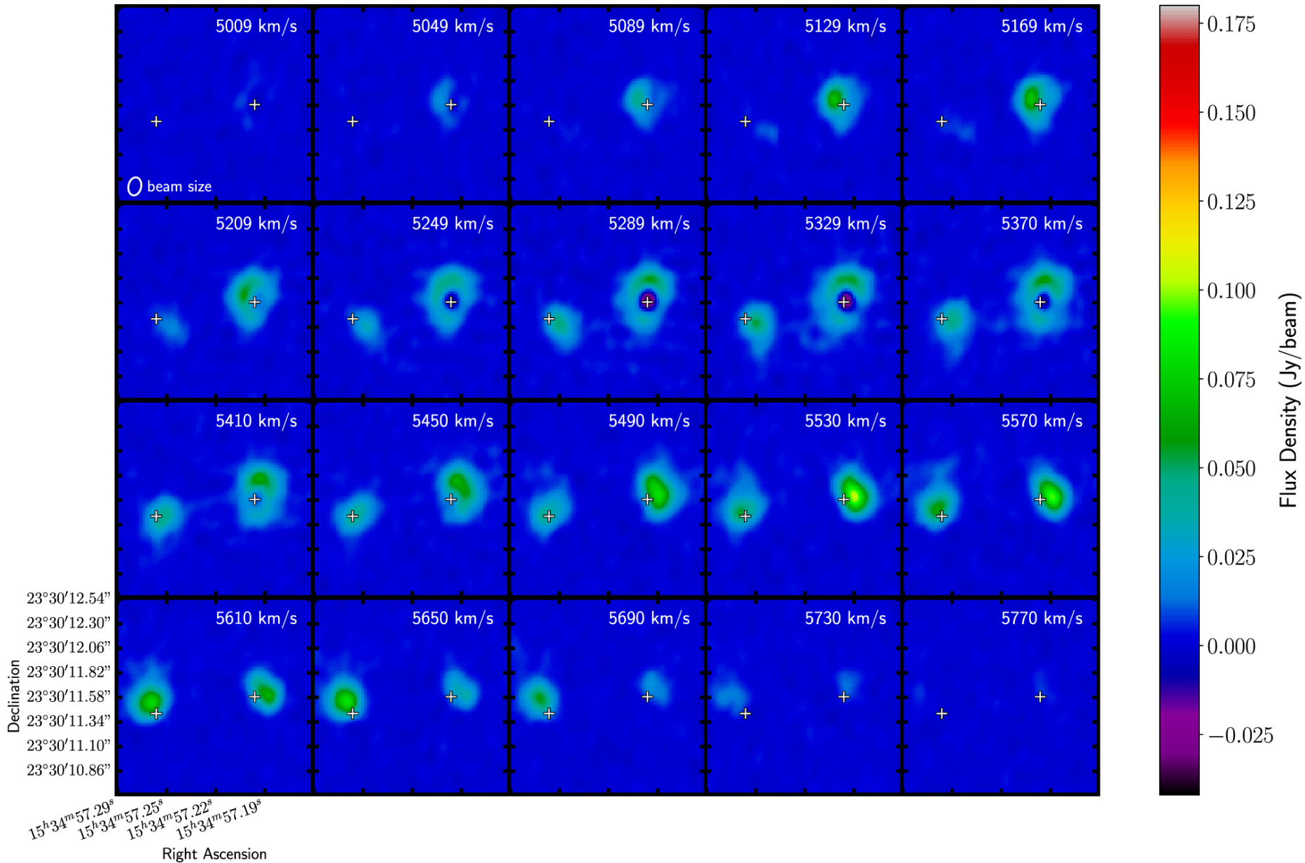
Figure 4. from Arp 220: New Observational Insights into the Structure and Kinematics of the Nuclear Molecular Disks and Surrounding Gas null 2020 APJ 896 43 doi:10.3847/1538-4357/ab8f32 https://dx.doi.org/10.3847/1538-4357/ab8f32 © 2020. The American Astronomical Society. All rights reserved.
