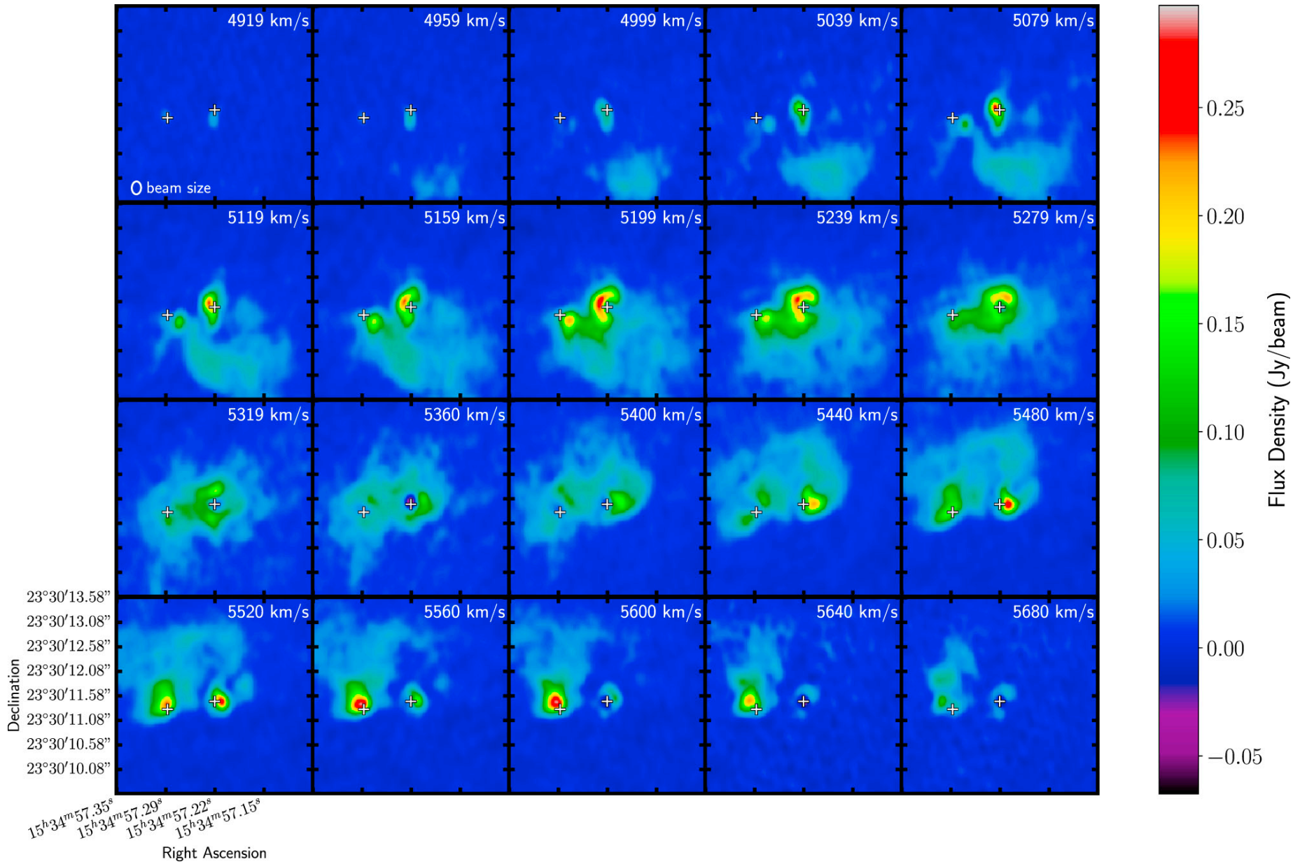
Figure 2. from Arp 220: New Observational Insights into the Structure and Kinematics of the Nuclear Molecular Disks and Surrounding Gas null 2020 APJ 896 43 doi:10.3847/1538-4357/ab8f32 https://dx.doi.org/10.3847/1538-4357/ab8f32 © 2020. The American Astronomical Society. All rights reserved.
