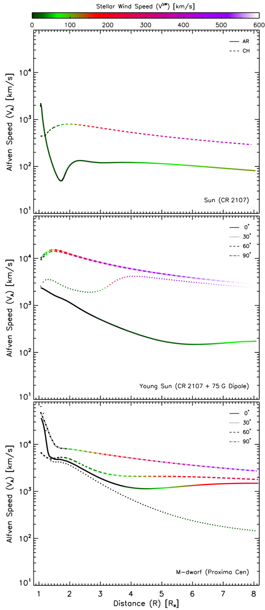
Figure 2. from Tuning the Exospace Weather Radio for Stellar Coronal Mass Ejections null 2020 APJ 895 47 doi:10.3847/1538-4357/ab88a3 http://dx.doi.org/10.3847/1538-4357/ab88a3 © 2020. The American Astronomical Society. All rights reserved.
