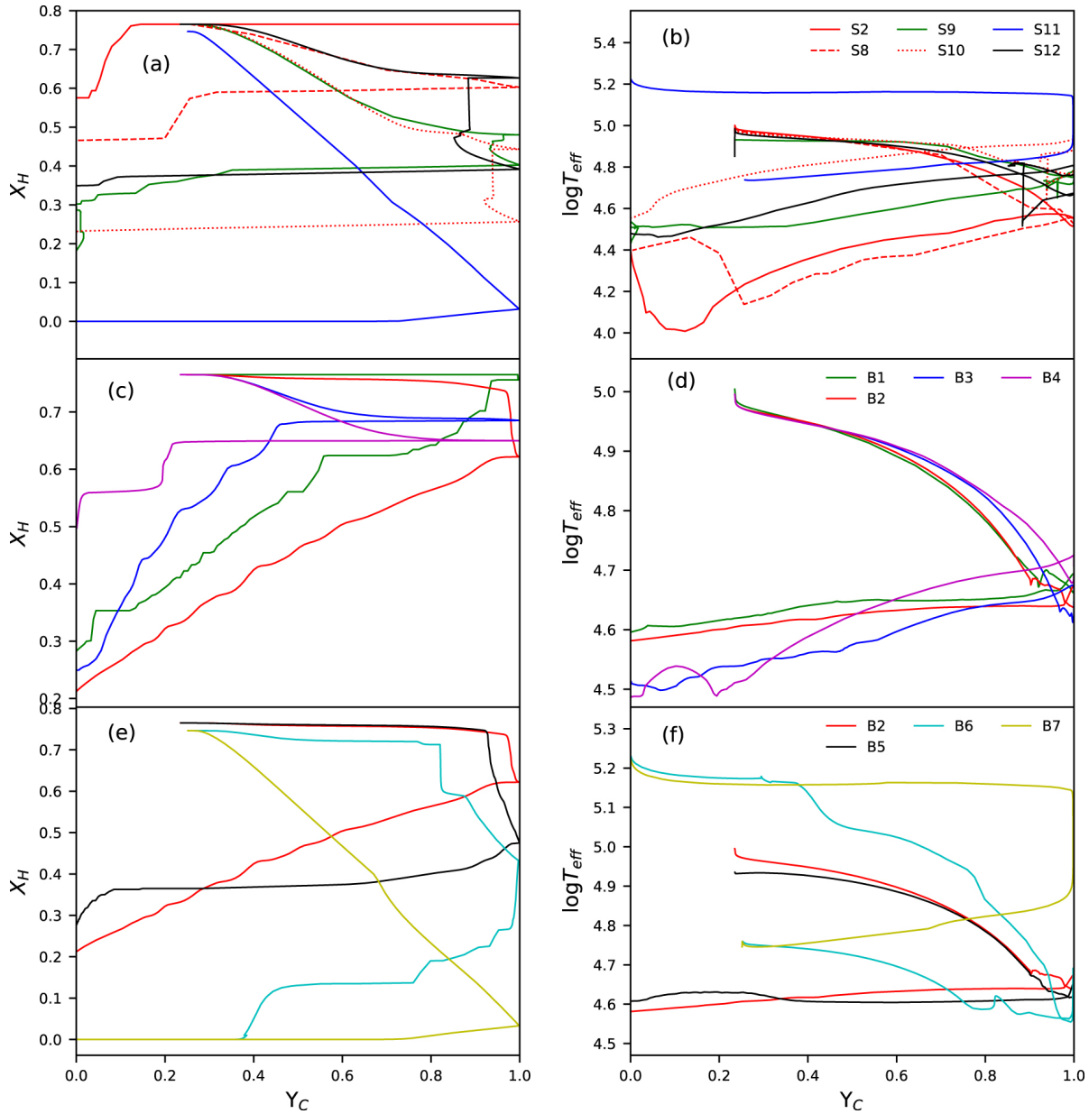
Figure 8. from The Structure and Evolution of Massive Rotating Single and Binary Population III Stars null 2020 APJ 892 41 doi:10.3847/1538-4357/ab7993 http://dx.doi.org/10.3847/1538-4357/ab7993
