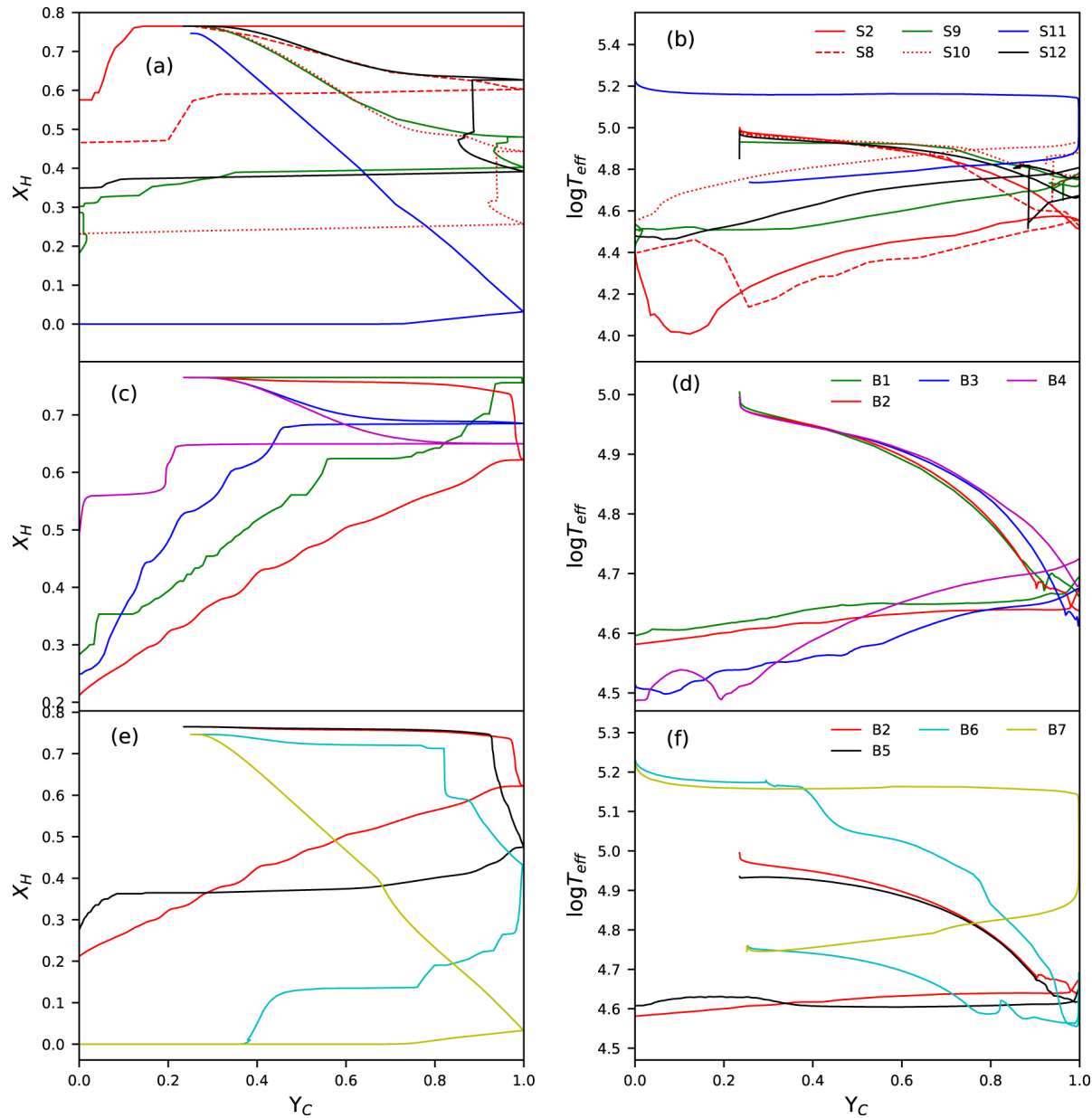
Figure 8. from The Structure and Evolution of Massive Rotating Single and Binary Population III Stars null 2020 APJ 892 41 doi:10.3847/1538-4357/ab7993 https://dx.doi.org/10.3847/1538-4357/ab7993 © 2020. The American Astronomical Society. All rights reserved.
