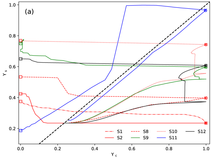
Figure 7. from The Structure and Evolution of Massive Rotating Single and Binary Population III Stars null 2020 APJ 892 41 doi:10.3847/1538-4357/ab7993 http://dx.doi.org/10.3847/1538-4357/ab7993
