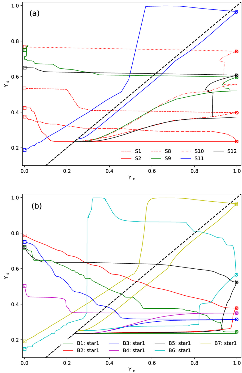
Figure 7. from The Structure and Evolution of Massive Rotating Single and Binary Population III Stars null 2020 APJ 892 41 doi:10.3847/1538-4357/ab7993 https://dx.doi.org/10.3847/1538-4357/ab7993 © 2020. The American Astronomical Society. All rights reserved.
