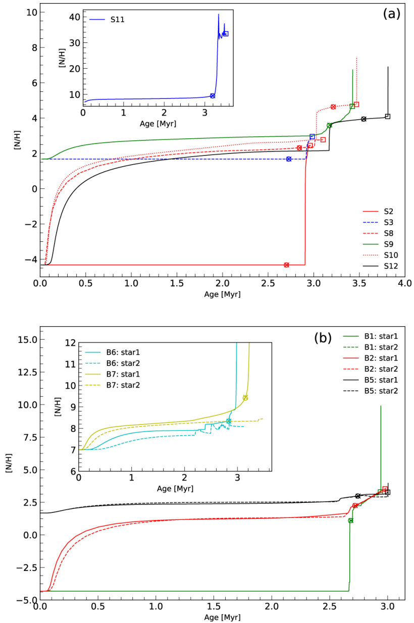
Figure 6. from The Structure and Evolution of Massive Rotating Single and Binary Population III Stars null 2020 APJ 892 41 doi:10.3847/1538-4357/ab7993 http://dx.doi.org/10.3847/1538-4357/ab7993 © 2020. The American Astronomical Society. All rights reserved.
