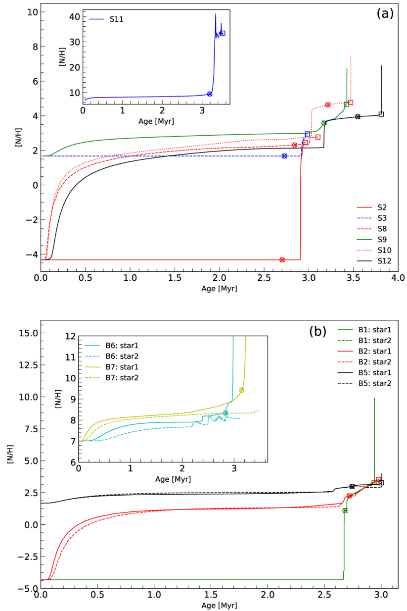
Figure 6. from The Structure and Evolution of Massive Rotating Single and Binary Population III Stars null 2020 APJ 892 41 doi:10.3847/1538-4357/ab7993 https://dx.doi.org/10.3847/1538-4357/ab7993 © 2020. The American Astronomical Society. All rights reserved.
