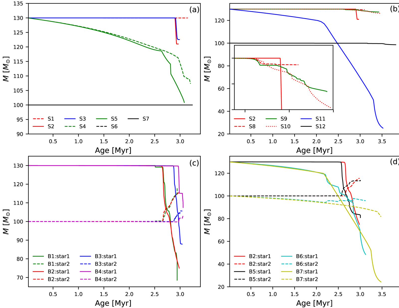
Figure 4. from The Structure and Evolution of Massive Rotating Single and Binary Population III Stars null 2020 APJ 892 41 doi:10.3847/1538-4357/ab7993 http://dx.doi.org/10.3847/1538-4357/ab7993
