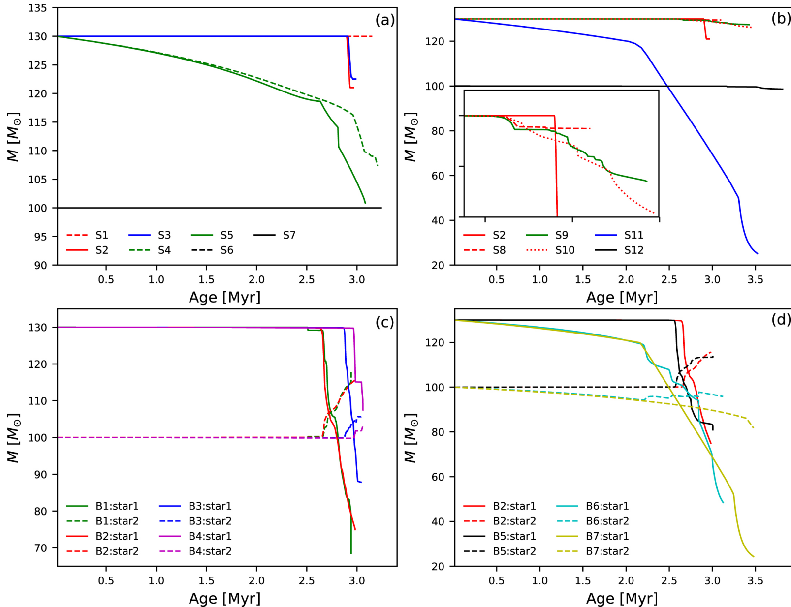
Figure 4. from The Structure and Evolution of Massive Rotating Single and Binary Population III Stars null 2020 APJ 892 41 doi:10.3847/1538-4357/ab7993 https://dx.doi.org/10.3847/1538-4357/ab7993
