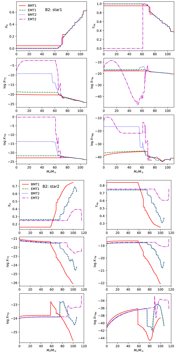
Figure 13. from The Structure and Evolution of Massive Rotating Single and Binary Population III Stars null 2020 APJ 892 41 doi:10.3847/1538-4357/ab7993 http://dx.doi.org/10.3847/1538-4357/ab7993
