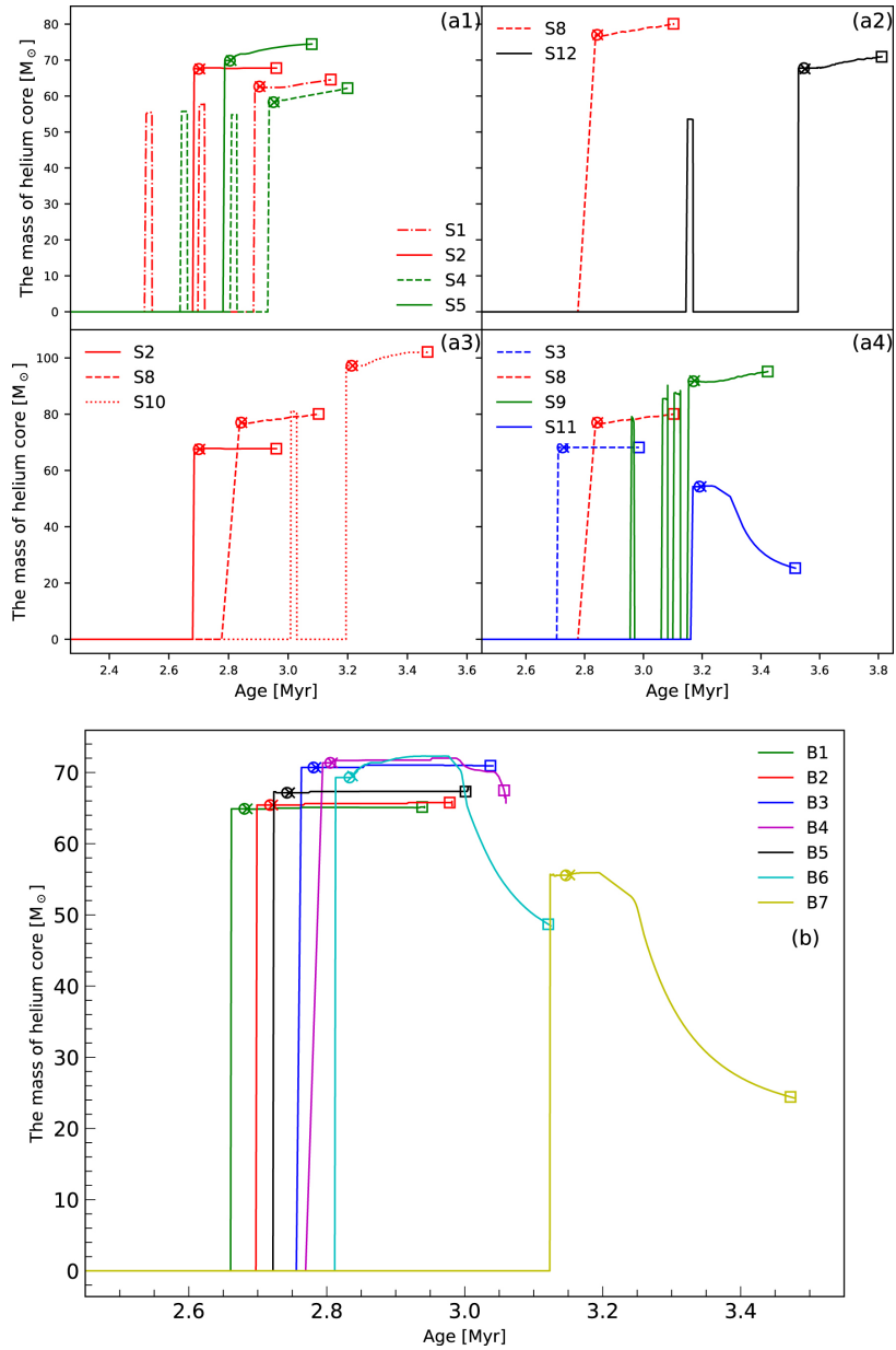
Figure 10. from The Structure and Evolution of Massive Rotating Single and Binary Population III Stars null 2020 APJ 892 41 doi:10.3847/1538-4357/ab7993 http://dx.doi.org/10.3847/1538-4357/ab7993
