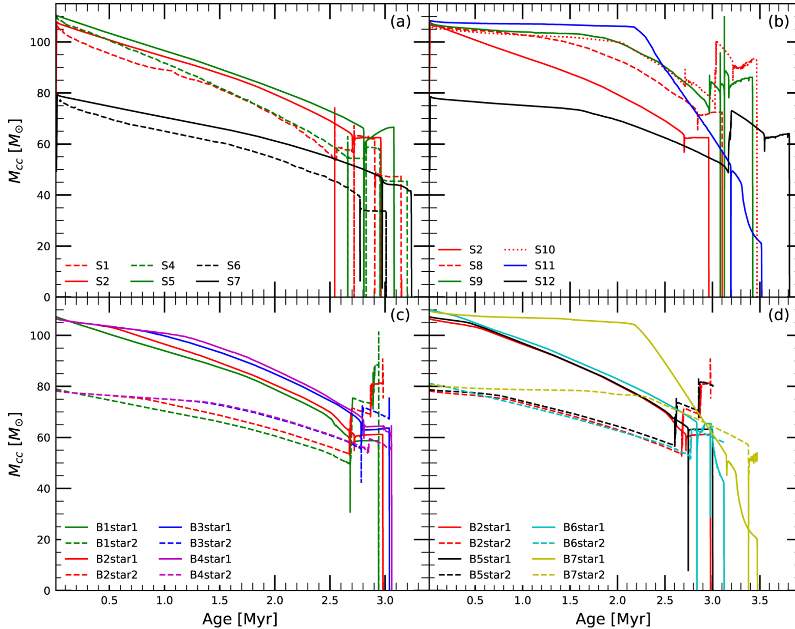
Figure 1. from The Structure and Evolution of Massive Rotating Single and Binary Population III Stars null 2020 APJ 892 41 doi:10.3847/1538-4357/ab7993 http://dx.doi.org/10.3847/1538-4357/ab7993 © 2020. The American Astronomical Society. All rights reserved.
