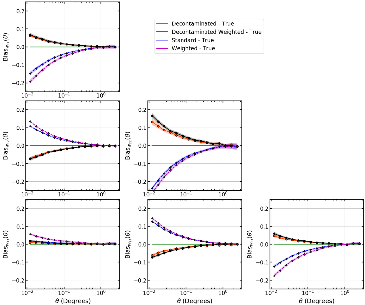
Figure 9. from Angular Correlation Function Estimators Accounting for Contamination from Probabilistic Distance Measurements null 2020 APJ 890 78 doi:10.3847/1538-4357/ab63c8 http://dx.doi.org/10.3847/1538-4357/ab63c8 © 2020. The American Astronomical Society. All rights reserved.
