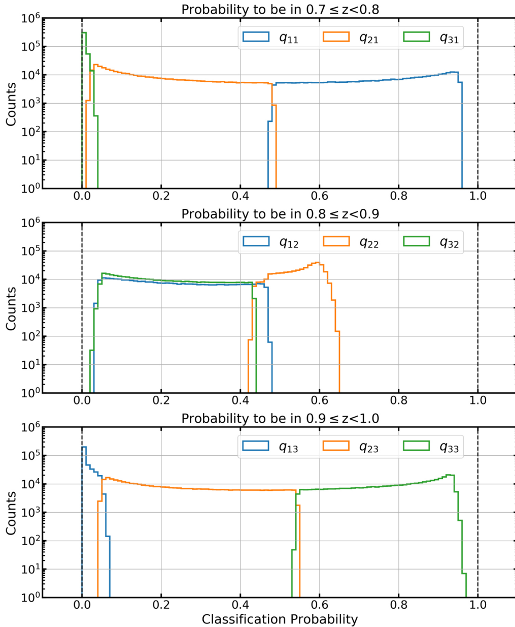
Figure 8. from Angular Correlation Function Estimators Accounting for Contamination from Probabilistic Distance Measurements null 2020 APJ 890 78 doi:10.3847/1538-4357/ab63c8 http://dx.doi.org/10.3847/1538-4357/ab63c8 © 2020. The American Astronomical Society. All rights reserved.
