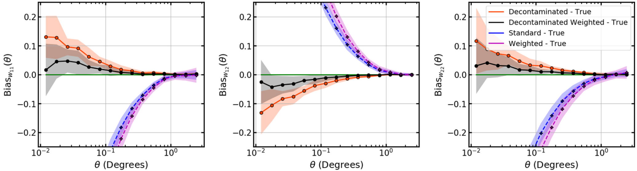
Figure 6. from Angular Correlation Function Estimators Accounting for Contamination from Probabilistic Distance Measurements null 2020 APJ 890 78 doi:10.3847/1538-4357/ab63c8 http://dx.doi.org/10.3847/1538-4357/ab63c8 © 2020. The American Astronomical Society. All rights reserved.
