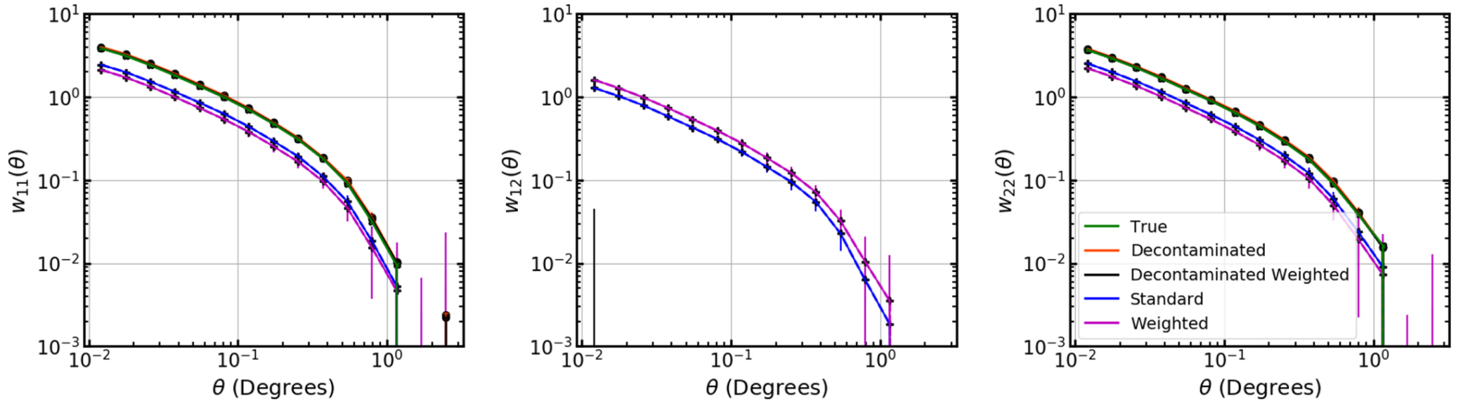
Figure 5. from Angular Correlation Function Estimators Accounting for Contamination from Probabilistic Distance Measurements null 2020 APJ 890 78 doi:10.3847/1538-4357/ab63c8 http://dx.doi.org/10.3847/1538-4357/ab63c8 © 2020. The American Astronomical Society. All rights reserved.
