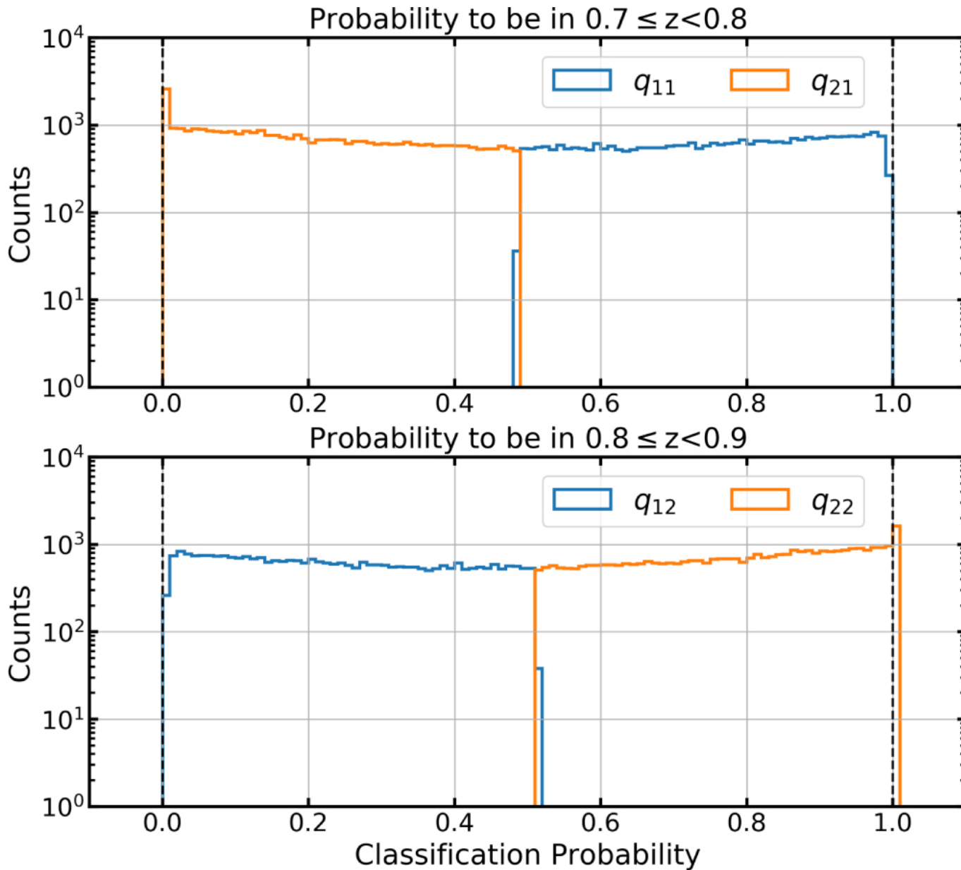
Figure 4. from Angular Correlation Function Estimators Accounting for Contamination from Probabilistic Distance Measurements null 2020 APJ 890 78 doi:10.3847/1538-4357/ab63c8 http://dx.doi.org/10.3847/1538-4357/ab63c8 © 2020. The American Astronomical Society. All rights reserved.
