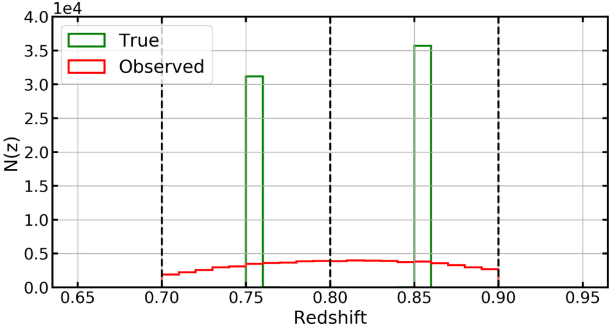
Figure 3. from Angular Correlation Function Estimators Accounting for Contamination from Probabilistic Distance Measurements null 2020 APJ 890 78 doi:10.3847/1538-4357/ab63c8 http://dx.doi.org/10.3847/1538-4357/ab63c8 © 2020. The American Astronomical Society. All rights reserved.
