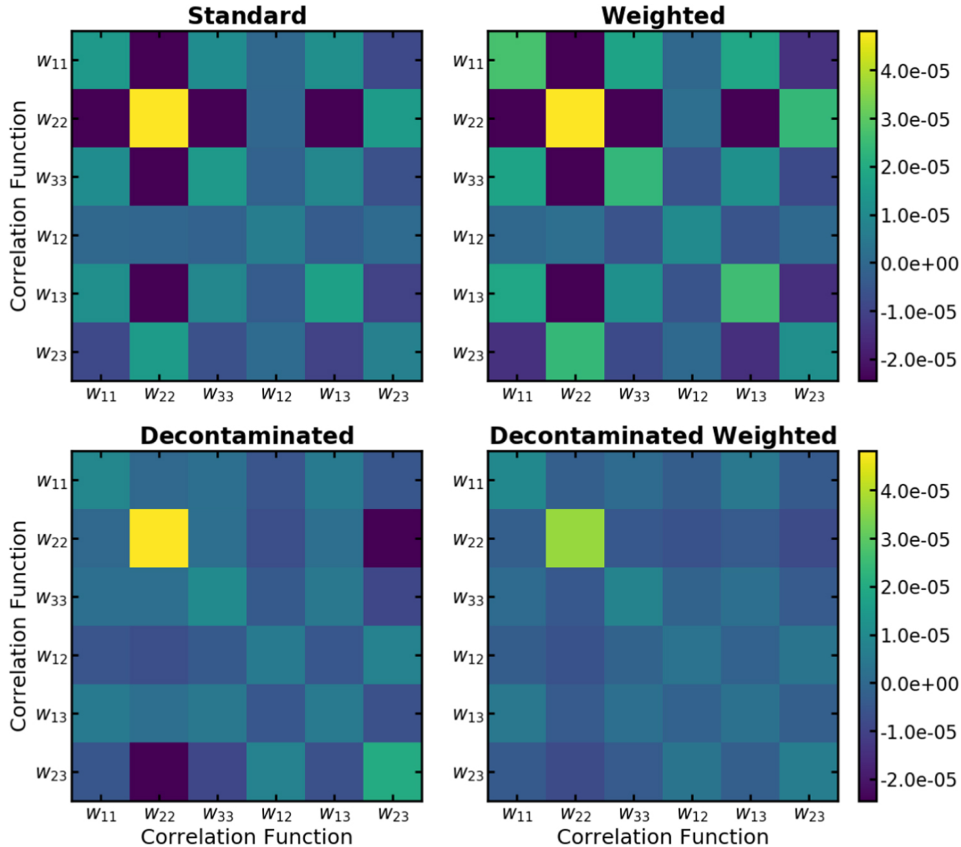
Figure 10. from Angular Correlation Function Estimators Accounting for Contamination from Probabilistic Distance Measurements null 2020 APJ 890 78 doi:10.3847/1538-4357/ab63c8 http://dx.doi.org/10.3847/1538-4357/ab63c8 © 2020. The American Astronomical Society. All rights reserved.
