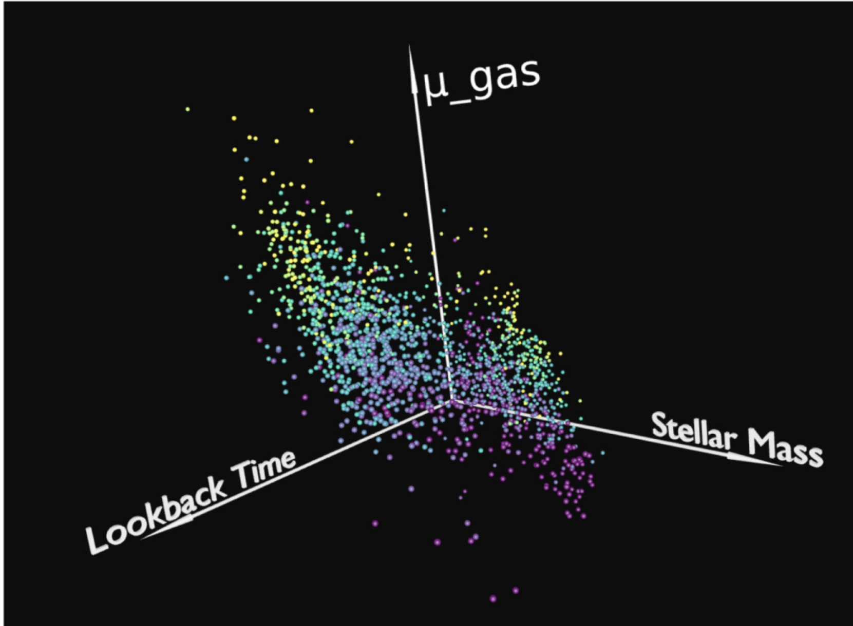
Figure 7. from Automated Mining of the ALMA Archive in the COSMOS Field (A3COSMOS). II. Cold Molecular Gas Evolution out to Redshift 6 null 2019 APJ 887 235 doi:10.3847/1538-4357/ab578d https://dx.doi.org/10.3847/1538-4357/ab578d © 2019. The American Astronomical Society. All rights reserved.
